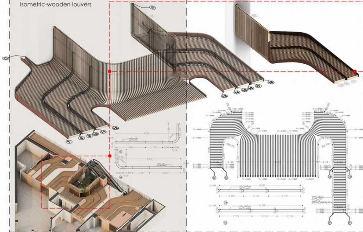
Isometric
