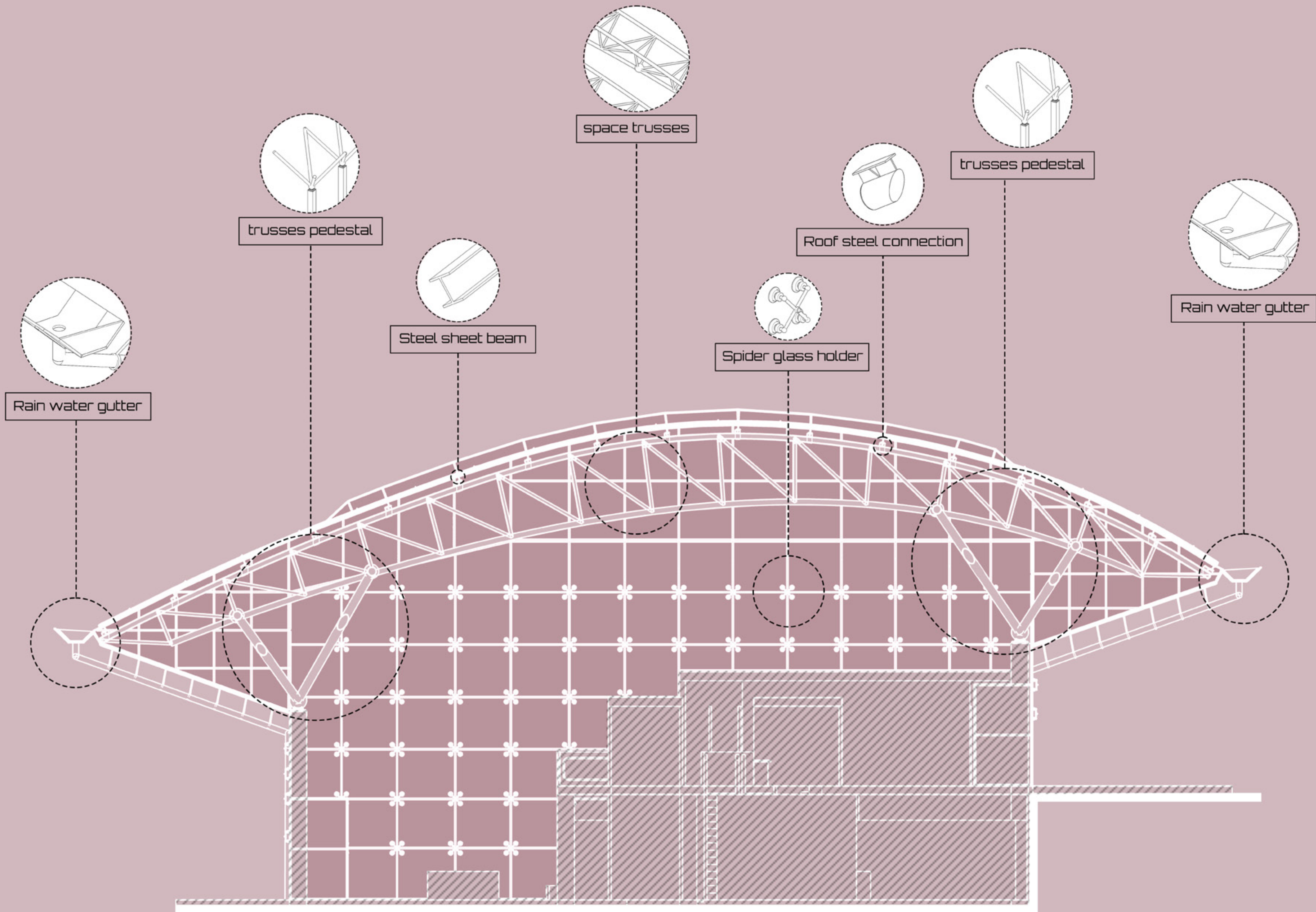
Roof structure section
